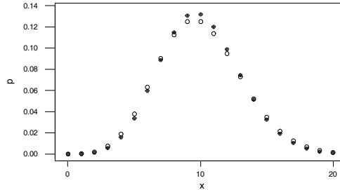
Figure 2.3.5: Plot of the \text{Binomial}(100, 1/10) (●●●) and the \text{Poisson}(10) (○○○) probability functions at the values 0, 1, \dots, 20 .
