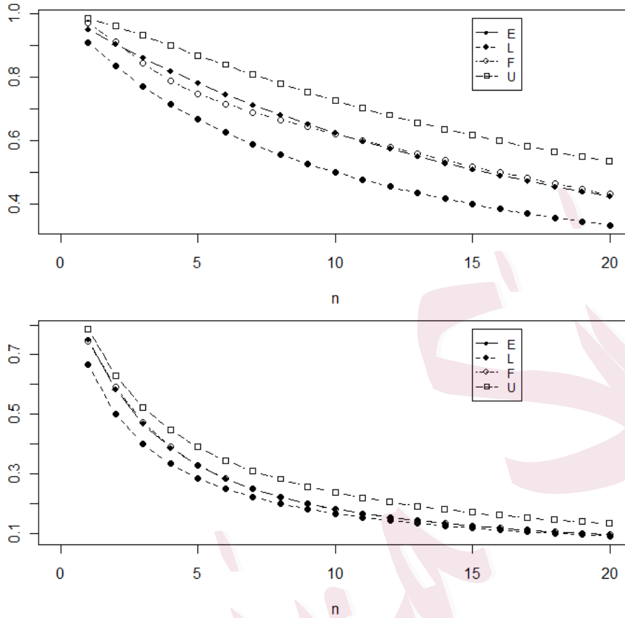
Figure 1: Comparison of inverse moment approximations for n = 1, 2, \dots, 20 and \theta = 0.1 (top) and \theta = 0.5 (bottom). The exact result (E) is obtained by Chao and Strawderman (1972), the leading term approximation (L) is given by Garcia and Palacios (2001) and Shi, Wu and Liu (2010), the fourth order approximation (F) is shown in (3.13), and the upper bound (U) is obtained by Pittenger (1990).
