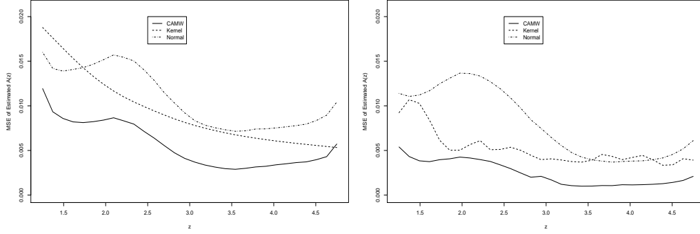
Figure 2: Simulation results with the same setting as Figure 1, except that the model has a Student- t error with 3 degree of freedom.
