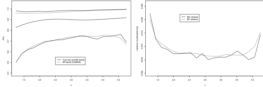
Figure 5: Simulation results with the same setting as Figure 4, except that the model has a Student- t error with 3 degree of freedom.
