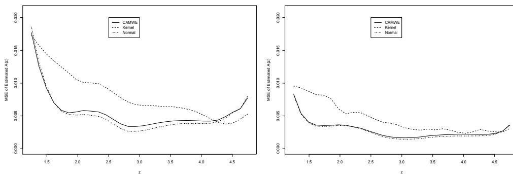
Figure 1: Simulation results for the model with normal error, where the sample sizes are m = n = 40 (left) and m = n = 100 (right), respectively. Shown are Monte Carlo averages of Mean Squared Errors (MSE) of three estimators, \hat{A}_M (CAMWE, solid), \hat{A}_N (Normal, dash-dotted) and \hat{A}_K (Kernel, dashed) at different values of z .
